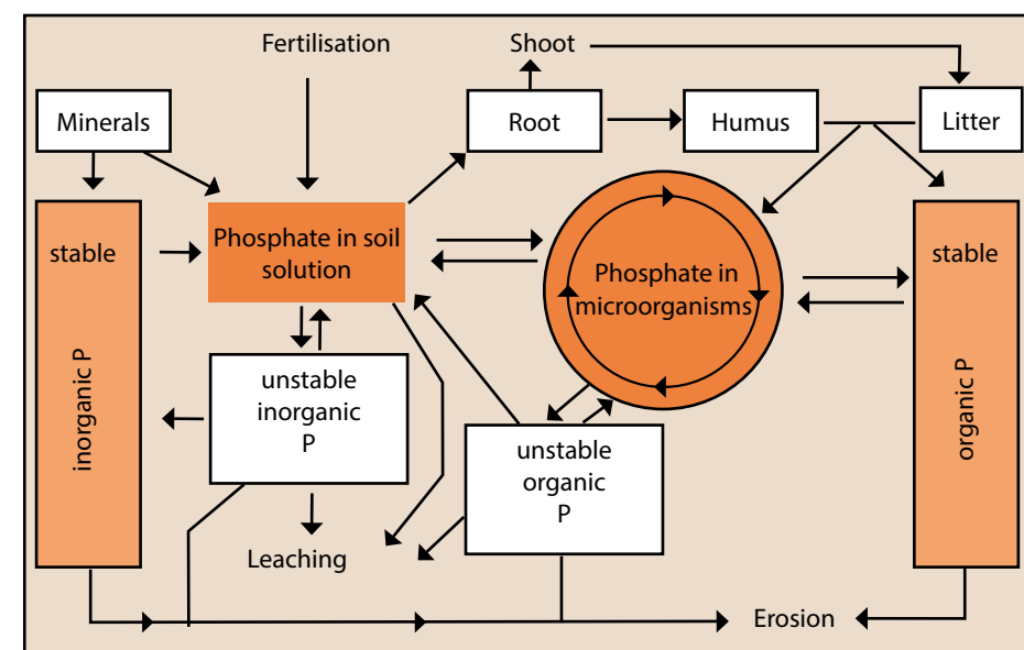
P cycle in the soil with the initial pools of the stable and unstable (labile) fractions (organic and inorganic) and the places of conversion: soil solution, microorganisms and plants [55]
